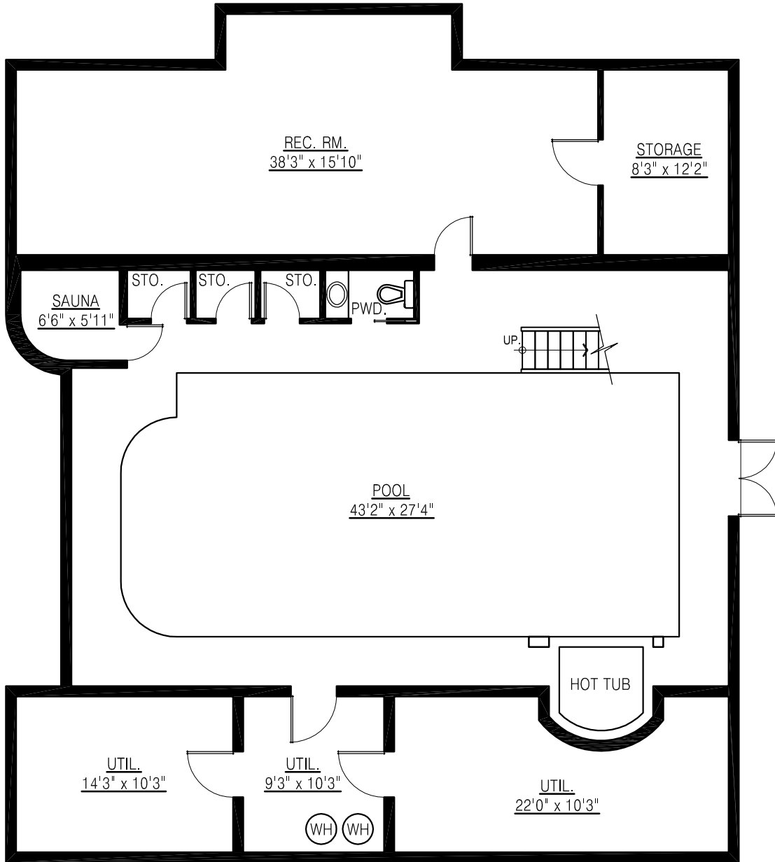
LOWER FLOOR PLAN FLOOR AREA: 2,521 sq.ft.
